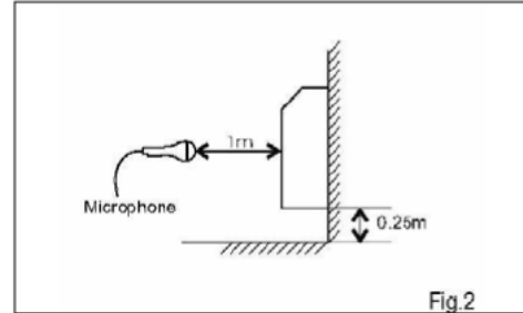
Figure 2. Floor Mounted
