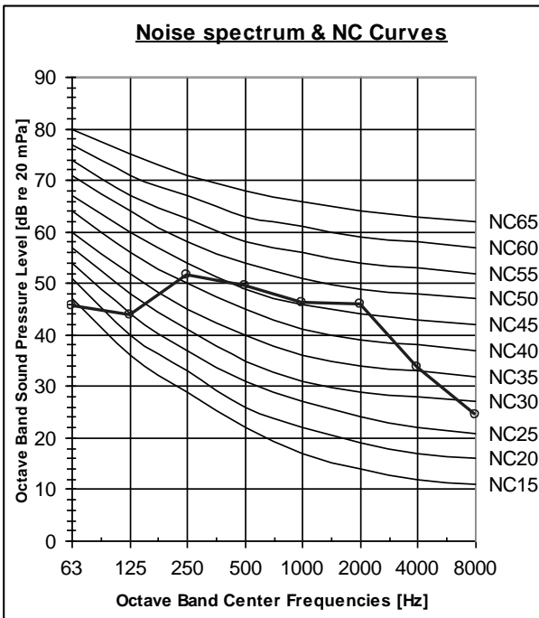
YGF024 Cooling
