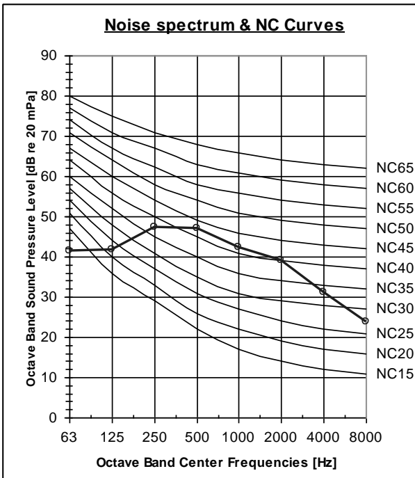
YGF007 Cooling
