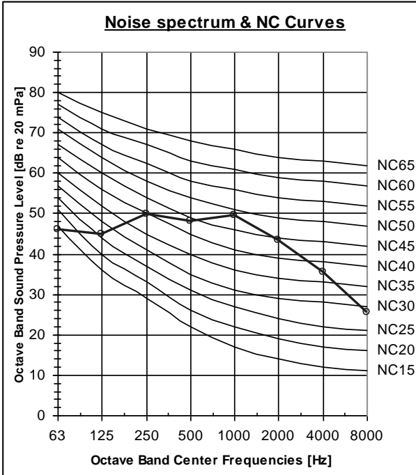
YGF018 Cooling
