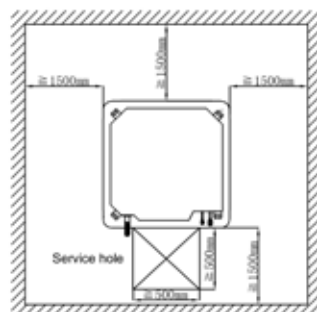
Installation space
