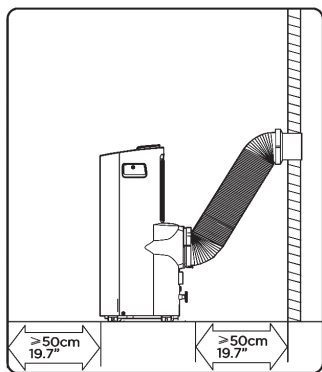
Wall installation
