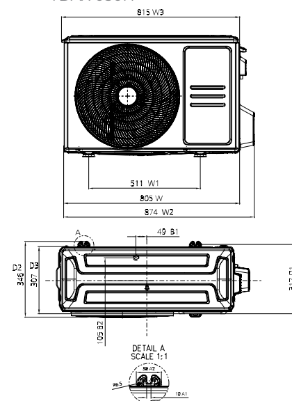
YDAX 050H
