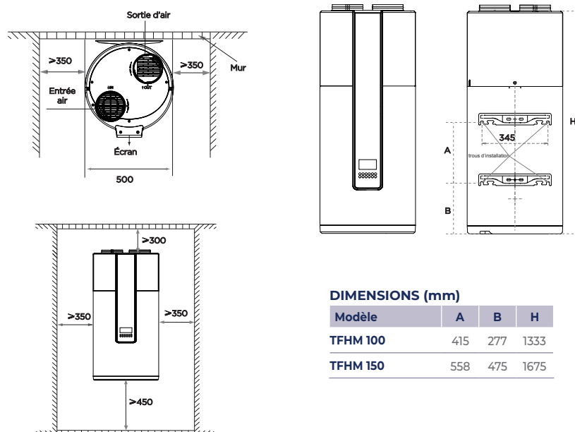
TFHM MURAL
