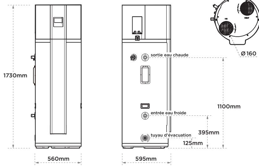
TFHM SOL
