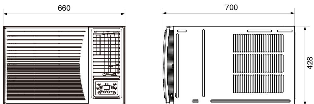
WFAE 035C
