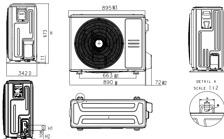
YDAX 140H
