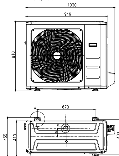
YDAX 90/100H
