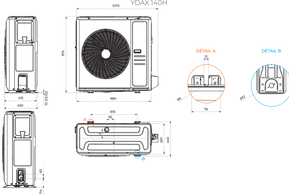
YDAX 140H
