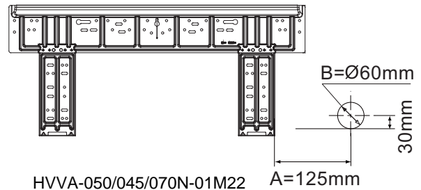
HVVA-050/045/070N-01M22
