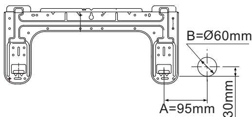
HVVA-025/022/035N-01M22
