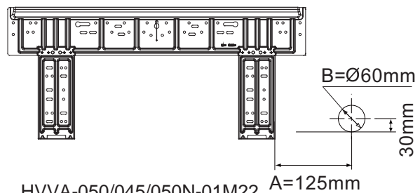
HVVA-050/045/050N-01M22
