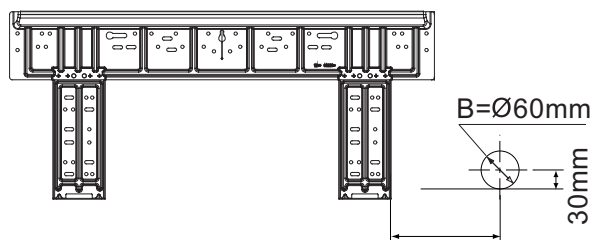
HVVA-045/050/070N-01M22
