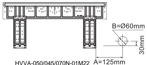
HVVA-050/045/070N-01M22
