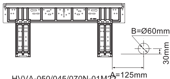
HVVA-050/045/070N-01M22
