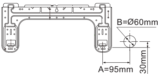
HVVA-025/022-35N-01M22
