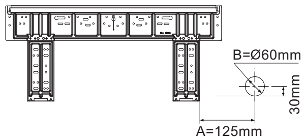
HVVA-050/045-70N-01M22
