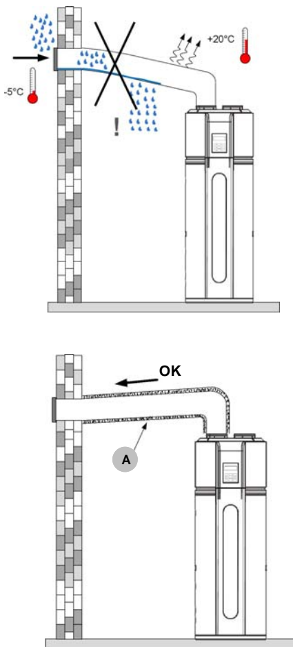
A - Insulated pipe
