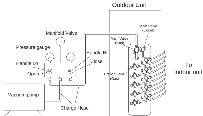
Vacuum outdoor unit YCZ327/YCZ430/YCZ542
