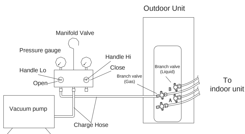
Vacuum outdoor unit YCZ218
