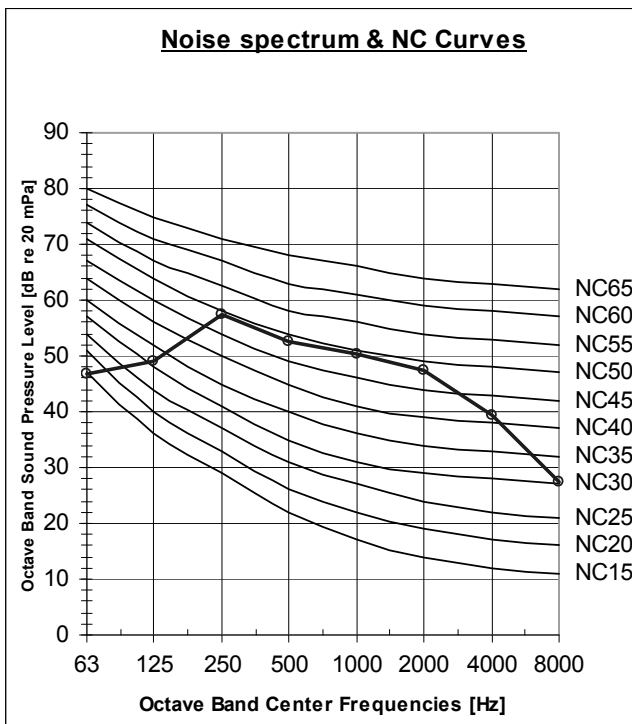
ELAU-VFF045-H13 Cooling
