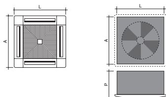
U.I.: AE ECF 9-11-15-18
