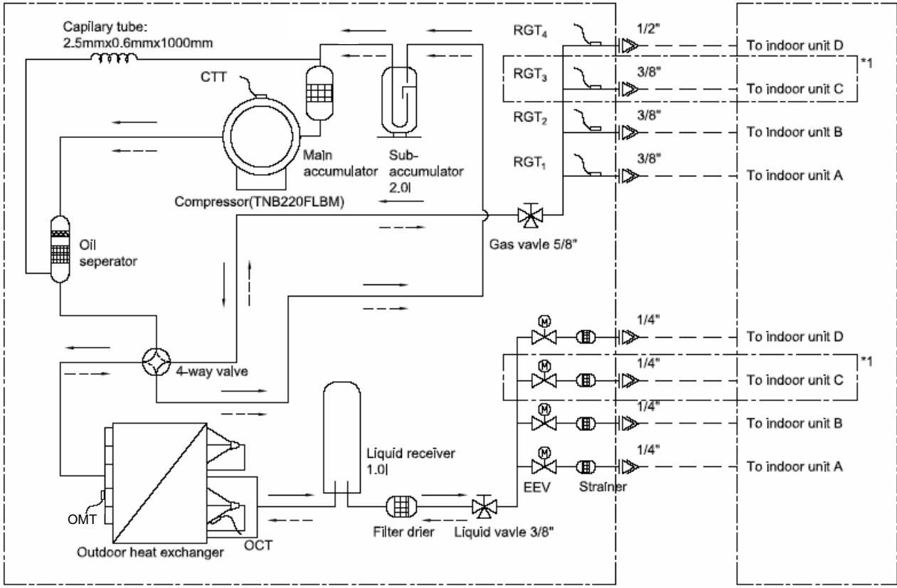
OUTDOOR UNIT
