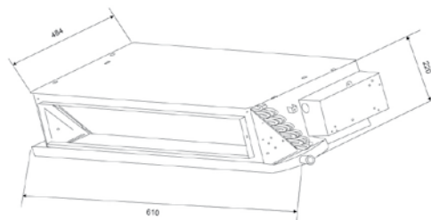
Dimensions: 009 model
