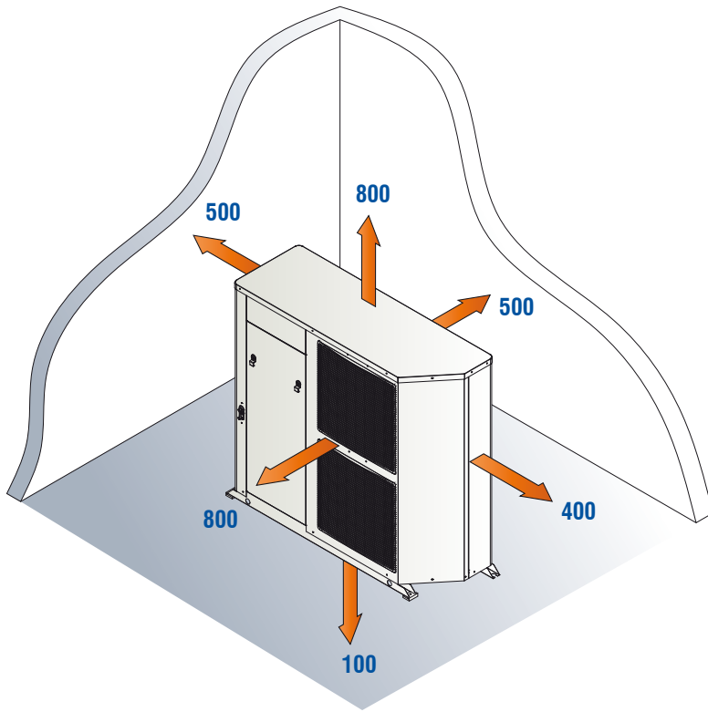
Outdoor unit
