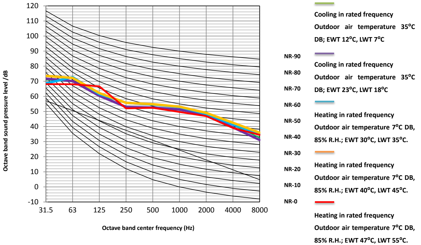
Figure 2-8.8: AW-WHPMA16-H91 octave band levels
