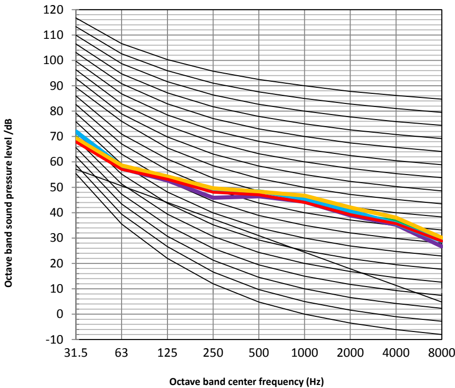
Figure 2-8.5: AW-WHPMA10-H91 octave band levels
