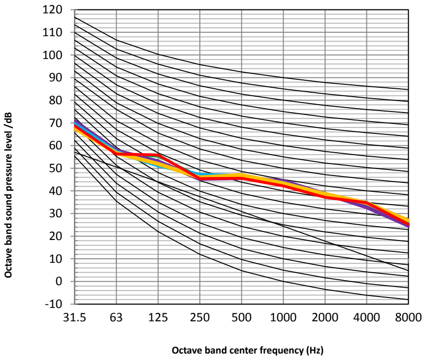
Figure 2-8.4: AW-WHPMA08-H91 octave band levels
