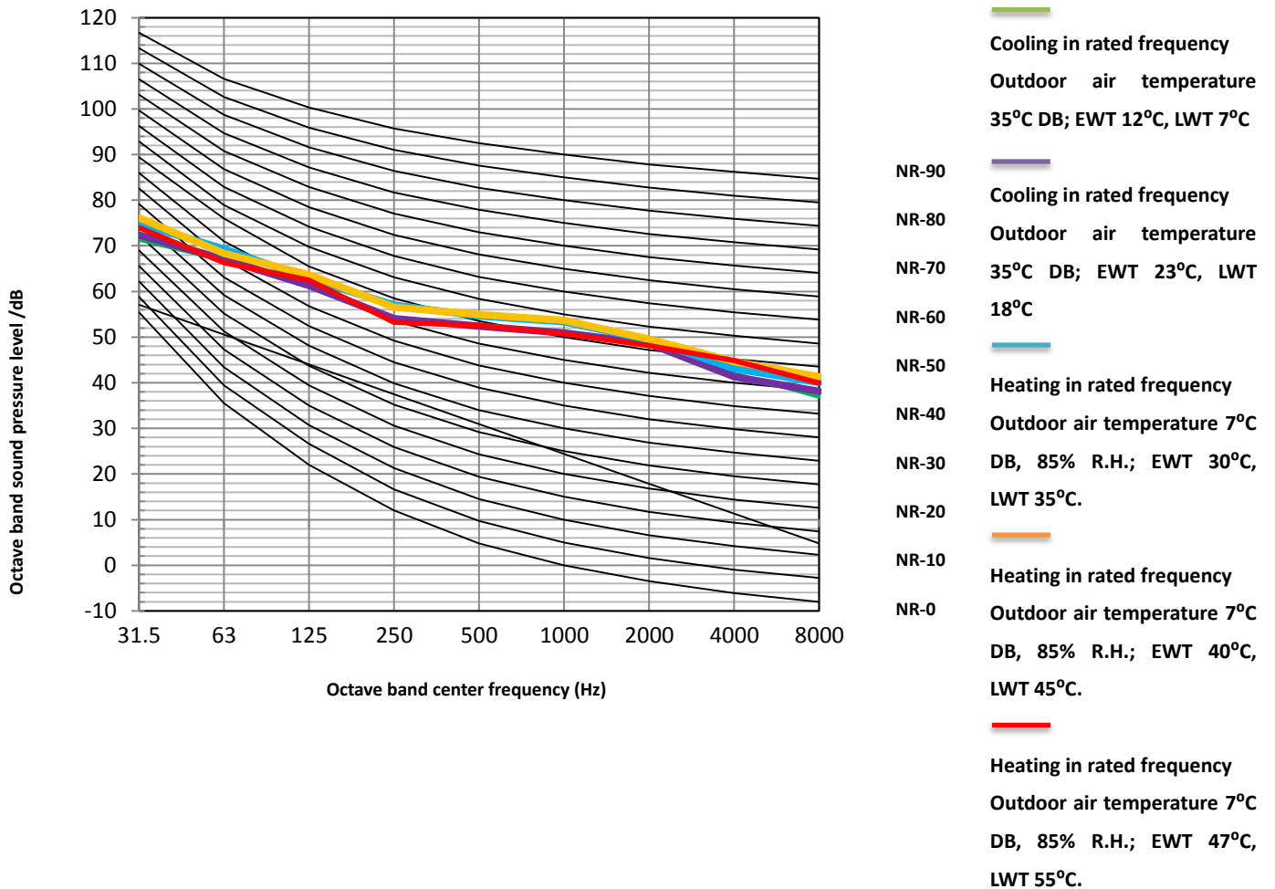
Figure 2-8.9: AW-WHPMA16-H93 octave band levels
