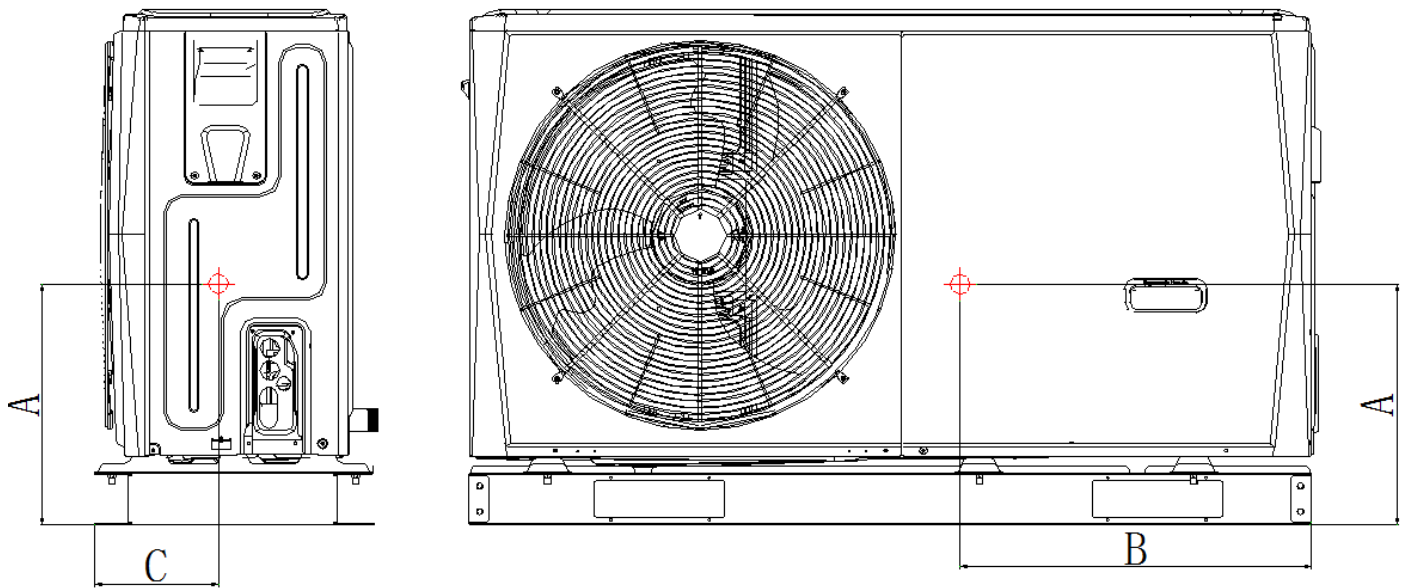
Figure 2-2.1: Wellea Mono 4/6 kW 1 phase dimensions and center of gravity (unit: mm)
