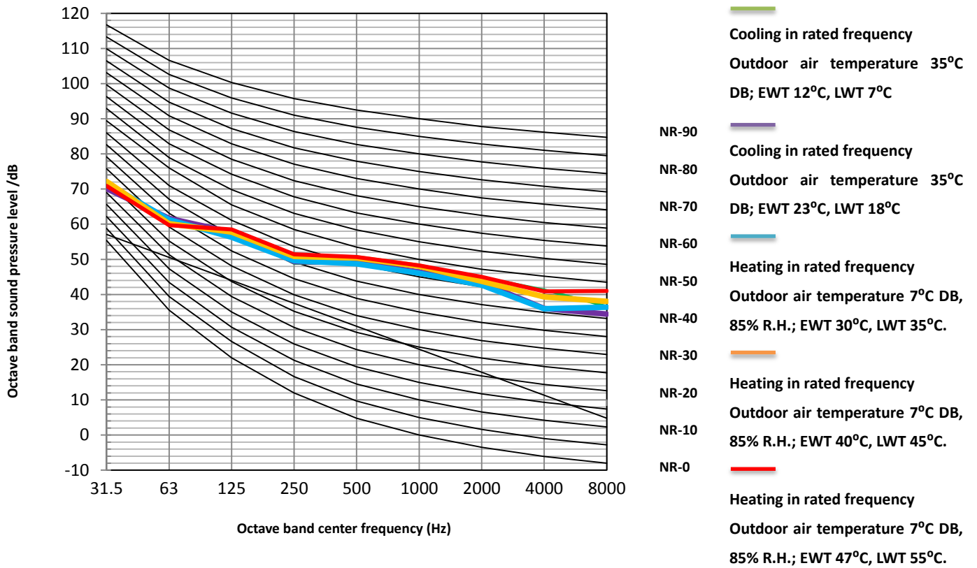
Figure 2-8.9: AW-WHPMA12-H93 octave band levels
