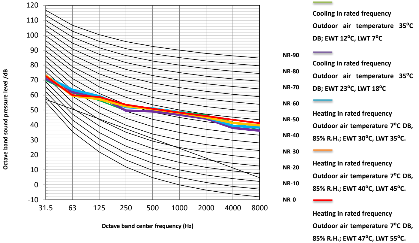
Figure 2-8.9: AW-WHPMA16-H93 octave band levels
