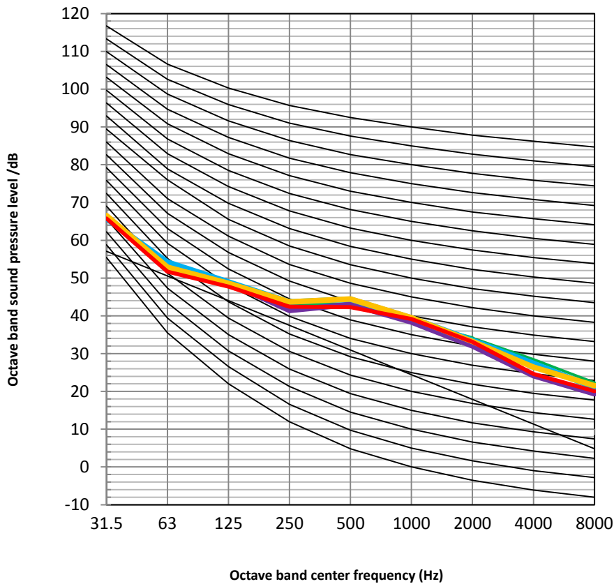
Figure 2-8.3: AW-WHPMA06-H91 octave band levels
