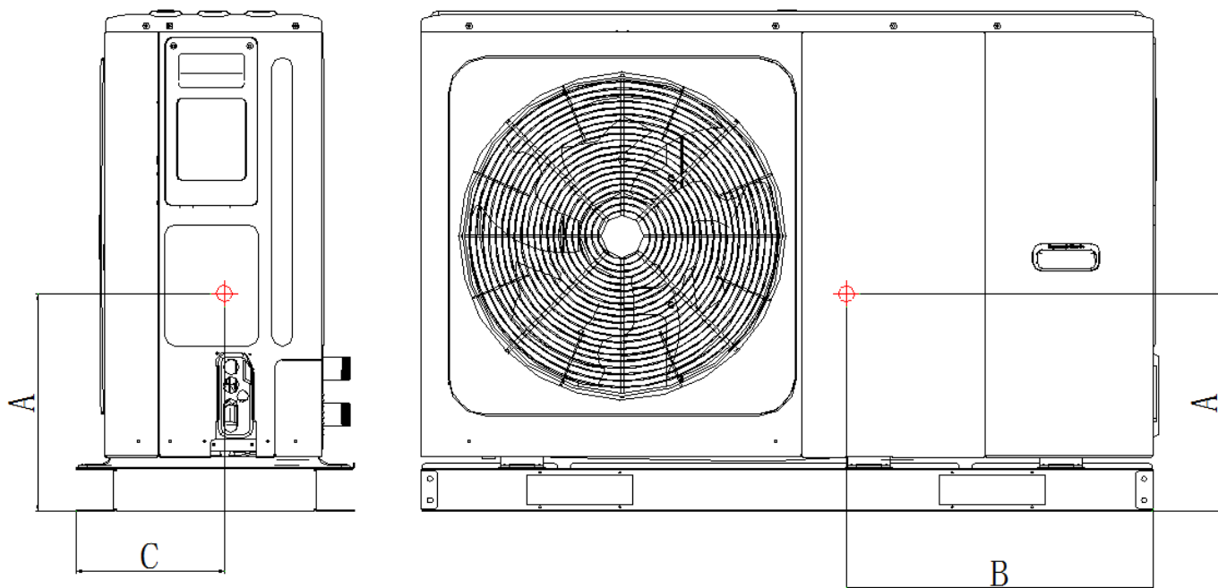
Figure 2-2.2: Wellea Mono 8/10/12/14/16 kW 1/3 phase(s) dimensions and center of gravity (unit: mm)
