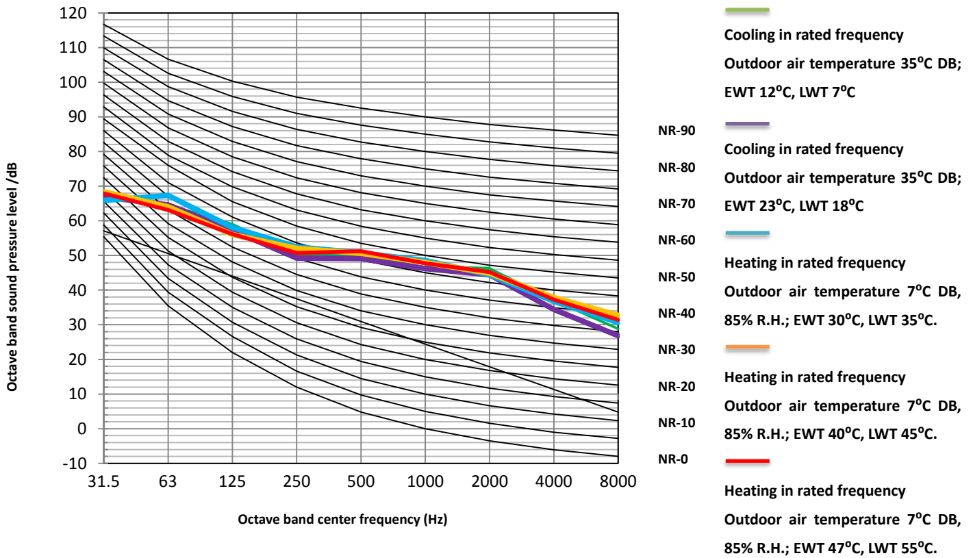
Figure 2-8.7: AW-WHPMA14-H91 octave band levels
