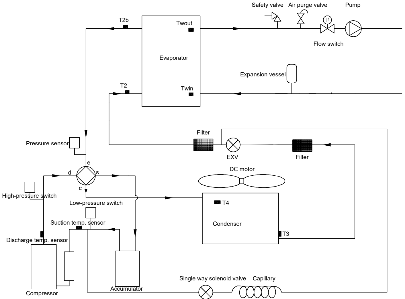
Figure 2-3.1: All sizes piping diagram
