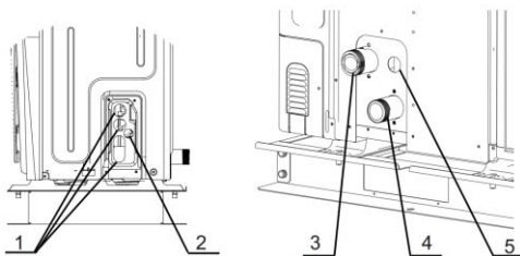
Figure 3-4.2: Wiring holes for 8~16kW models
