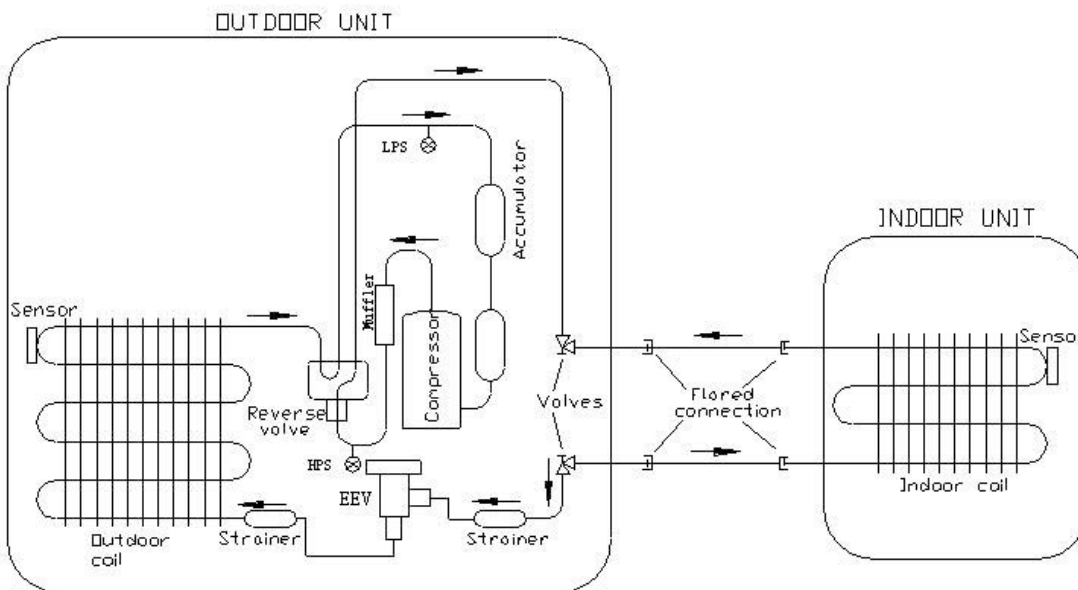
HEATING MODE
